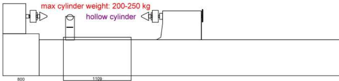
pneumatic end-tailstock and three-jaw chuck
